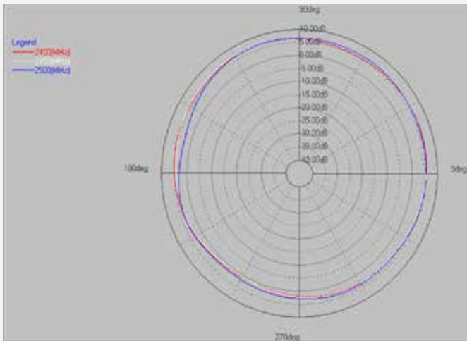
2.4G (PHI=0)
