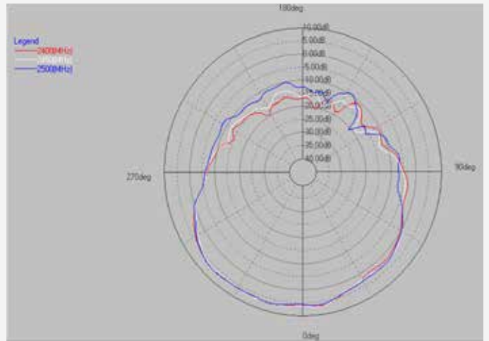
2.4G (PHI=90)
